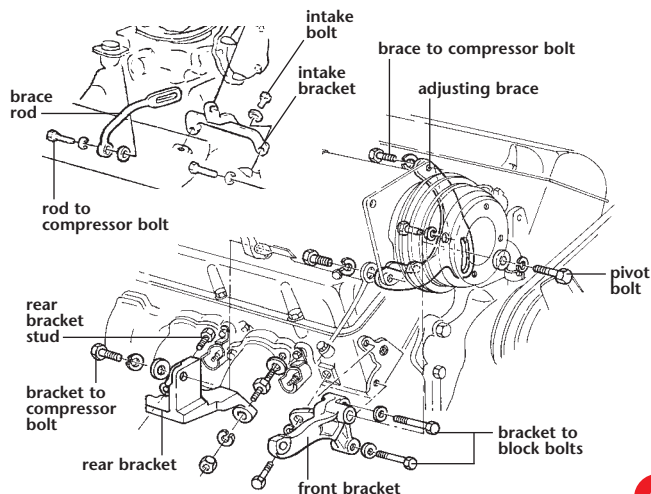
66-67 427 Compressor Mounting
