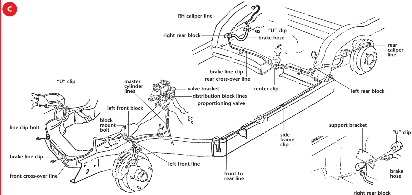
Rear Caliper Brake Lines
