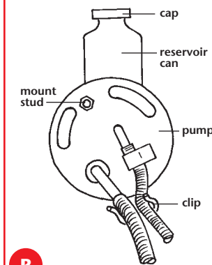
Power Steering Pump
