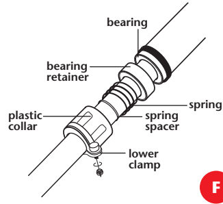
67-Late Lower Column
