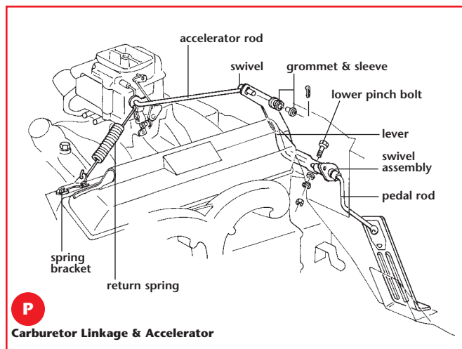
396 & 427 Carburetor Linkage
