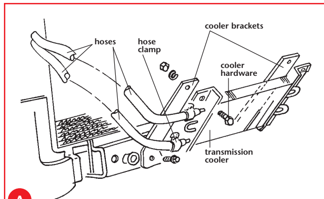
A Transmission Cooler
