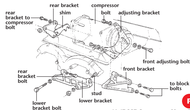
64-67 327 Compressor Mounting
