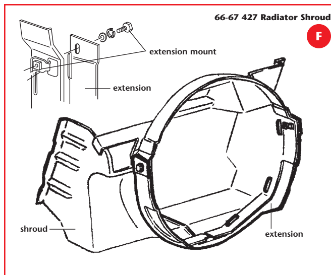
Radiator Shrouds
