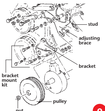
65-67 396 & 427 Pump Mounting
