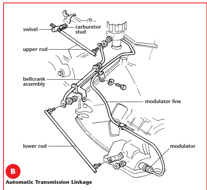
Transmission Kickdown Rods
