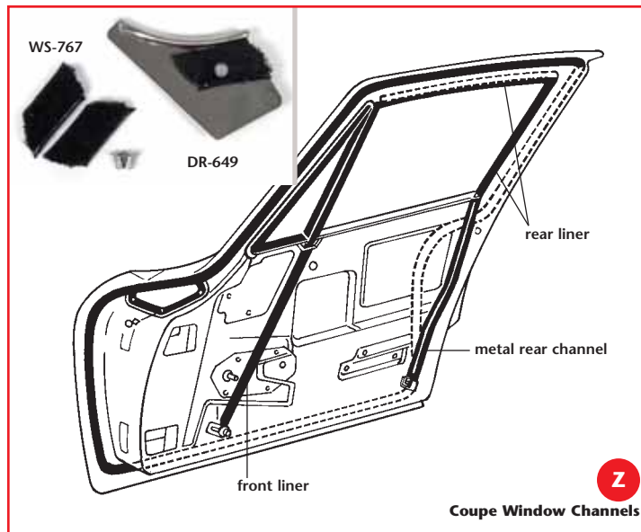
Coupe Window Channels & Liners
