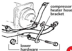
64-67 Compressor Hose Bracket
