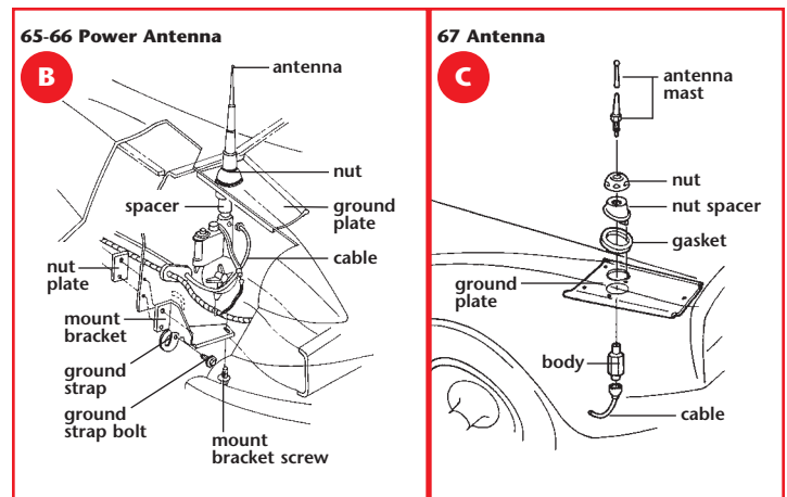
65-66 Power Antenna
