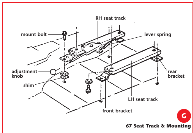
67 Seat Track & Mounting
