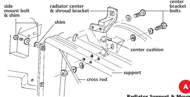
Radiator Support & Mount
