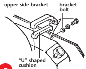
427 Radiator Mount to Support
